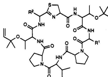
25 R 1 = R 2 = Leu 26 R 1 = Leu; R 2 = Val 27 R 1 = Val; R 2 = Phe
